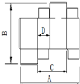
Single side pasting box
